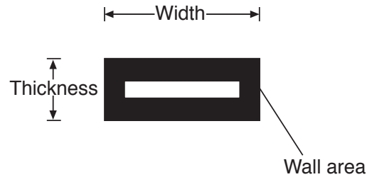
FIG. 1—Schematic diagram of the cross-section dimensions of fibres rewetted from handsheets.
